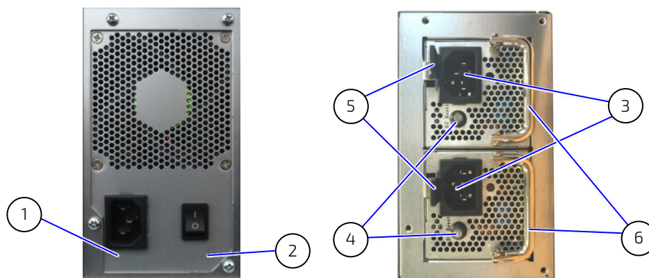
Figure 18: 600 W PSU or optional 500 W Redundant PSU
